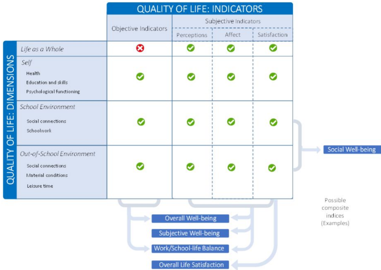
Figure 8.1. Framework overview
